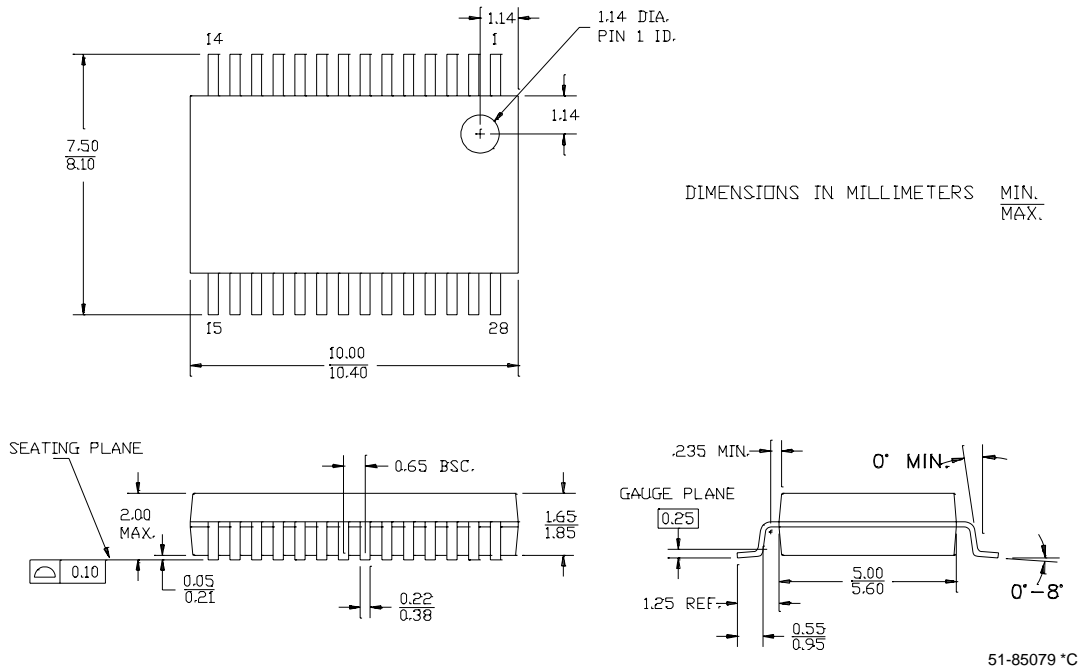
Figure 2-3. 28-Lead (210-Mil) SSOP
