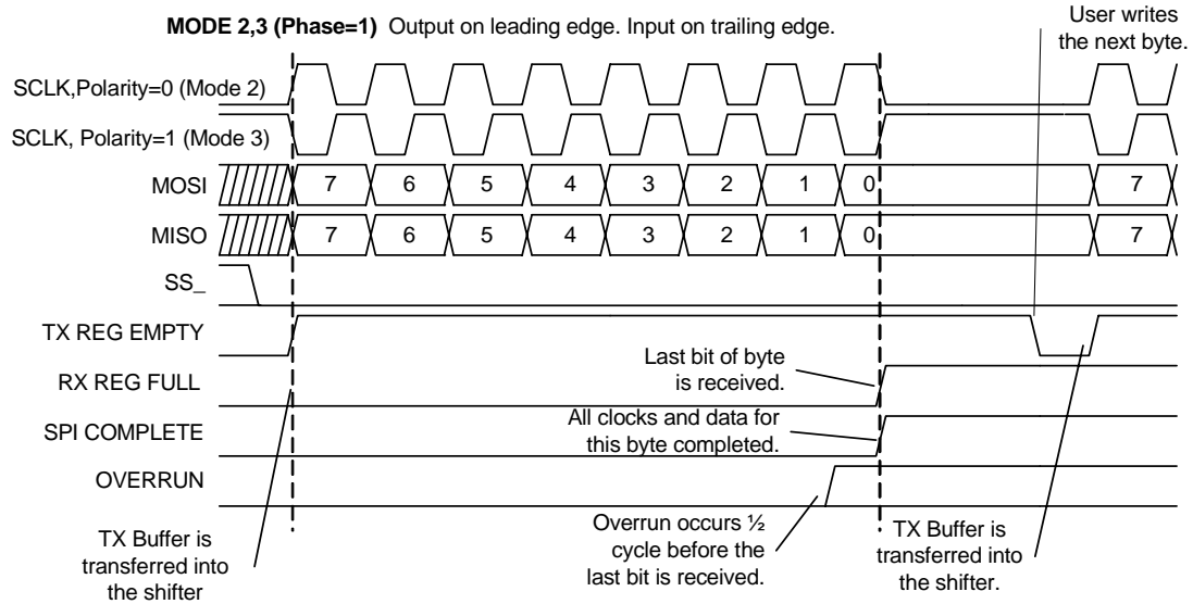
Figure 17-18. SPI Status Timing for Modes 2 and 3
