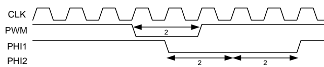
Figure 17-11. PWM Width Equal to Dead Band Period
