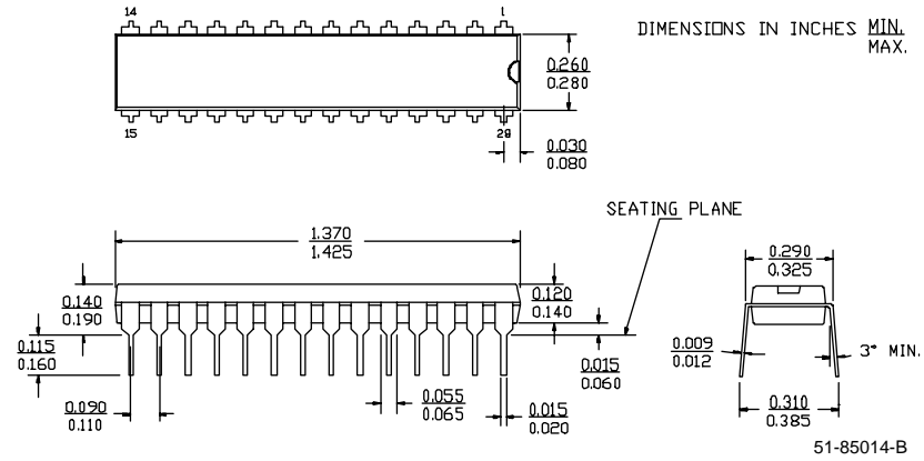
Figure 2-4. 28-Lead (300-Mil) Molded DIP
