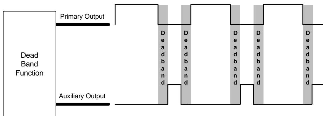
Figure 17-3. Dead Band Functional Overview
