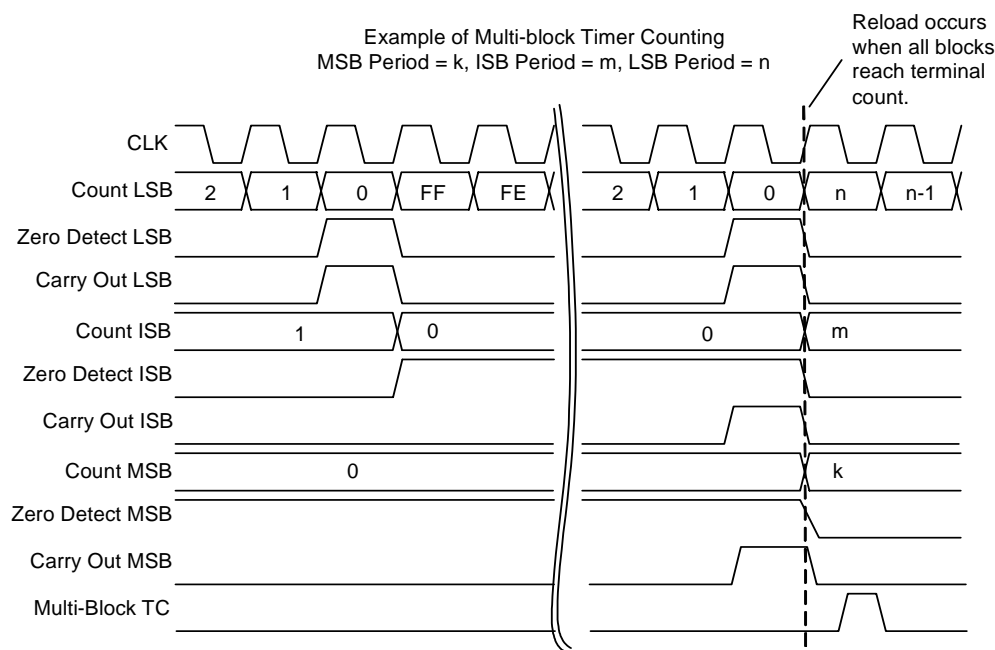
Figure 17-6. Multi-Block Timing
