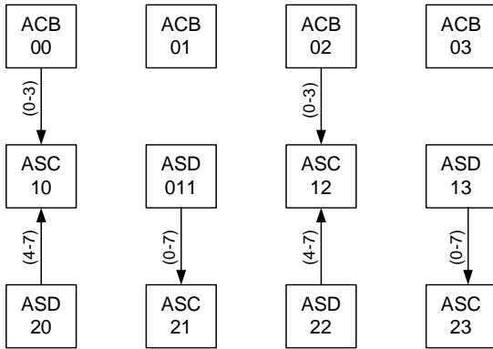
Figure 19-5. CMux Connections
