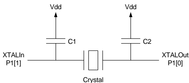
Figure 10-2. External Crystal Oscillator Connections
