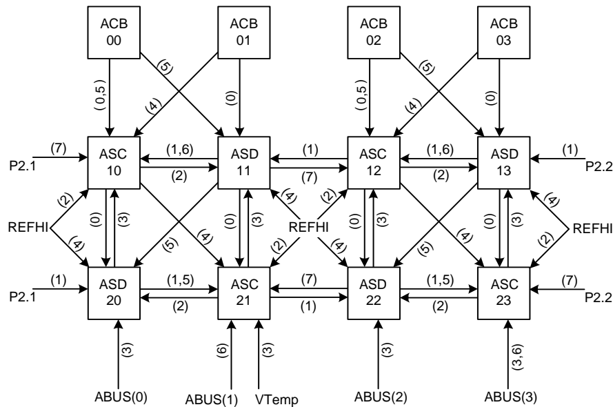
Figure 19-4. AMux Connections
