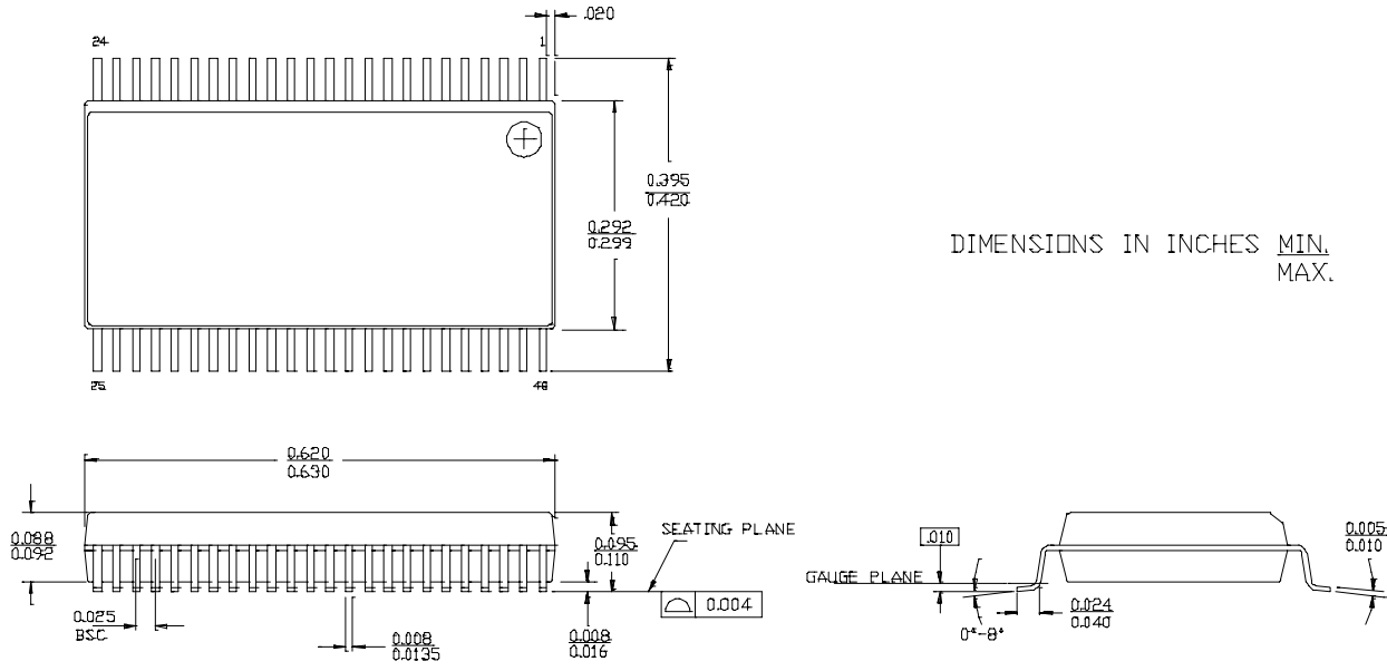
Figure 2-6. 48-Lead (300-Mil) SSOP
