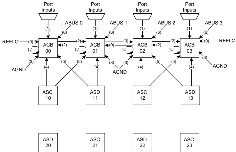
Figure 19-2. PMux Connections
