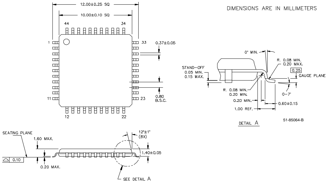
Figure 2-5. 44-Lead TQFP
