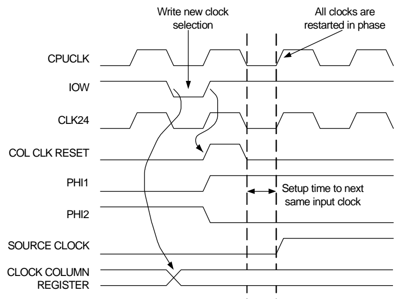
Figure 18-3. Column Clock Resynchronize on an IO Write
