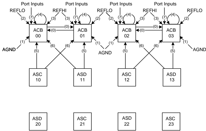
Figure 19-1. NMux Connections
