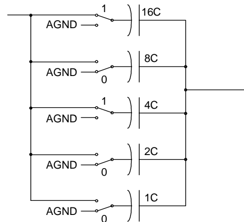
Figure 22-3. Example Switch Capacitor Settings
