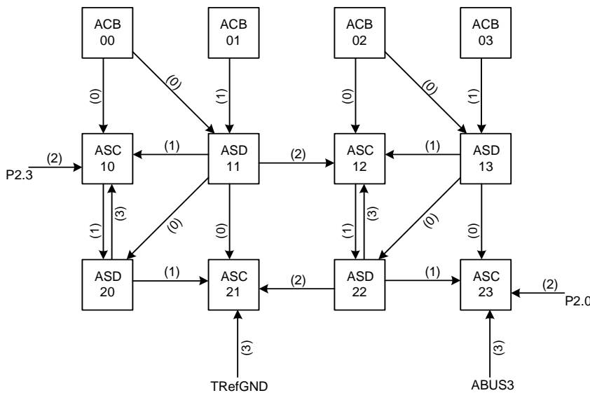
Figure 19-6. BMuxSC/SD Connections
