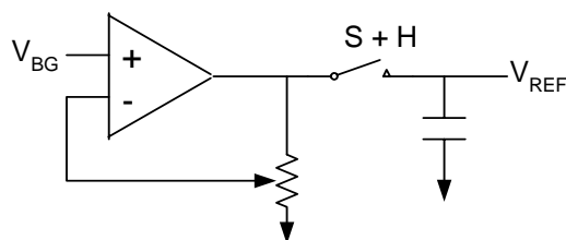
Figure 29-1. Voltage Reference Schematic
