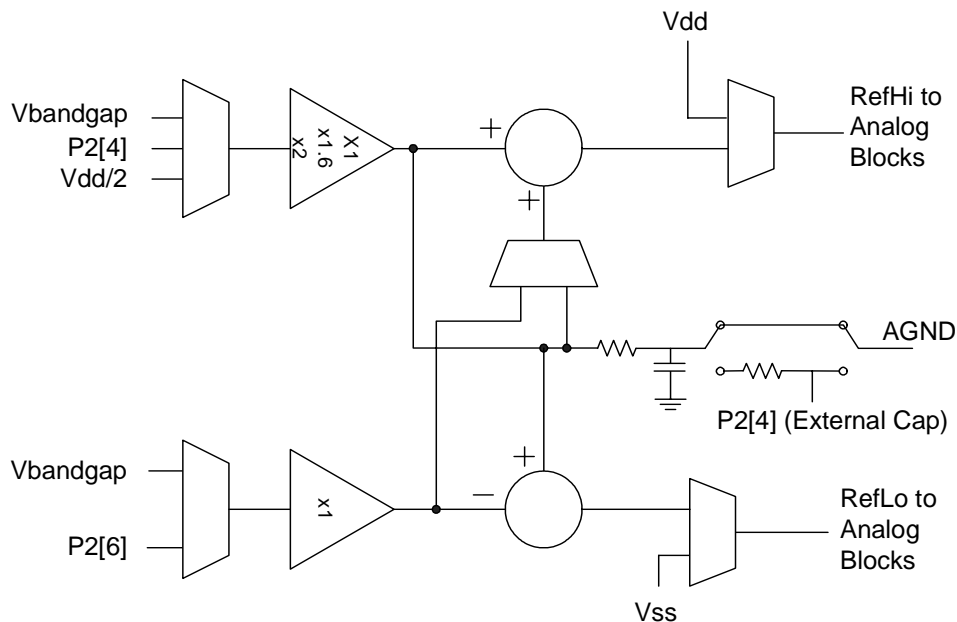
Figure 21-1. Analog Reference Control Schematic
