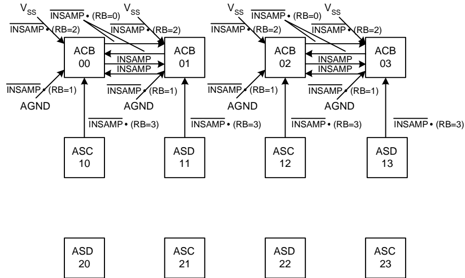
Figure 19-3. RBotMux Connections
