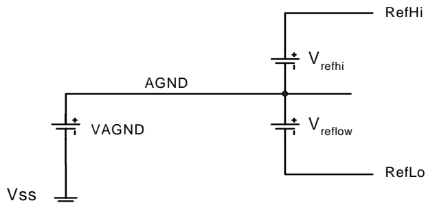
Figure 21-2. Reference Structure
