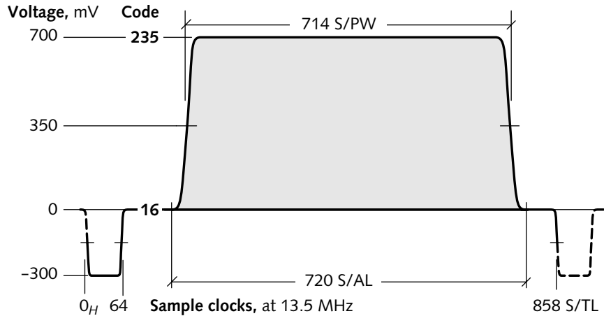
Figure 1.6 Scan line waveform for 525/59.94 component video, showing luma. The 720 active samples contain picture information. Horizontal blanking occupies the remaining sample intervals.
