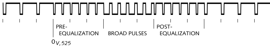
Figure 1.8 Vertical sync waveform of 525/59.94.
