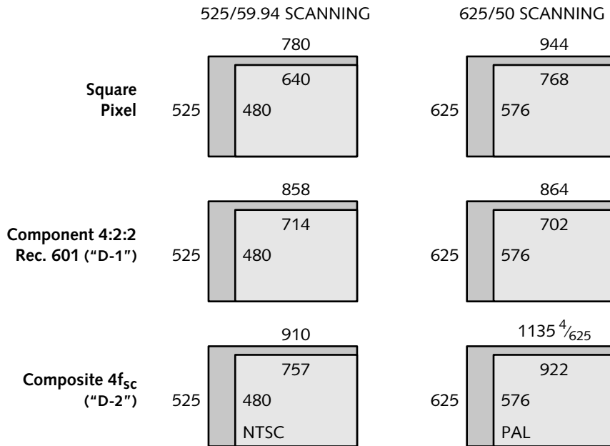
Figure 1.5 Digital video rasters. The left column shows 525/59.94 scanning, the right column shows 625/50. The top row shows sampling with square pixels. The middle row shows sampling at the Rec. 601 standard sampling frequency of 13.5 MHz. The bottom row shows sampling at four times the color subcarrier. Blanking intervals are shown with dark shading.
