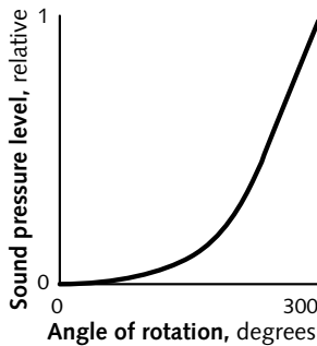
Figure 1.9 Audio taper.
