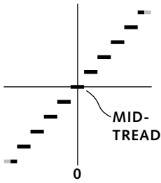
Figure 1.10 Mid-tread quantizer.
