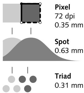
Figure 1.13 Pixel/spot/triad.
