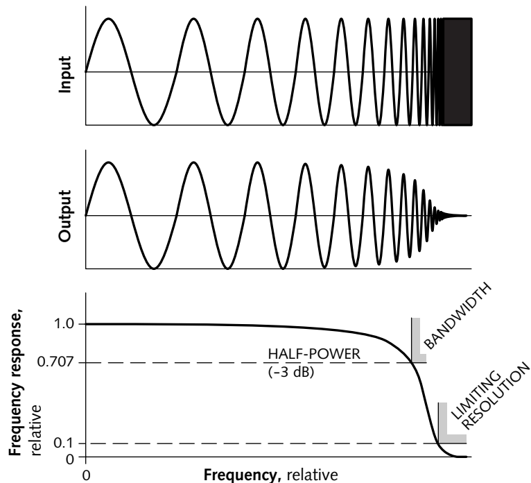
Figure 1.11 Frequency response of any electronic or optical system falls as frequency increases. Bandwidth is measured at the half-power point ( -3 dB), where response has fallen to 0.707. Television displays are often specified at limiting resolution , where response has fallen to 0.1.
